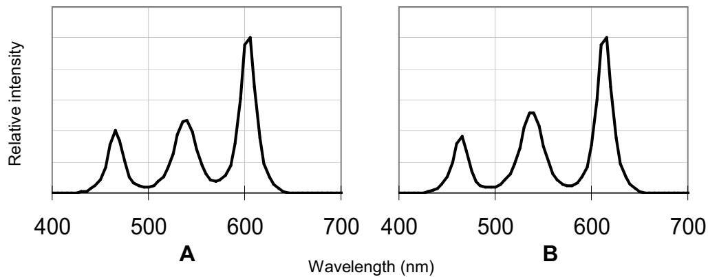
Figure 6: Spectral power distribution of modeled 3-color white LEDs with (A) peaks at 463, 538, and 603 nm and (B) peaks at 464, 538, and 613 nm.
