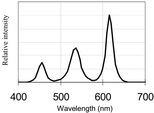
Figure 4: Spectral power distribution of modeled 3-color white LED, with peaks at 457, 534, and 616 nm.
